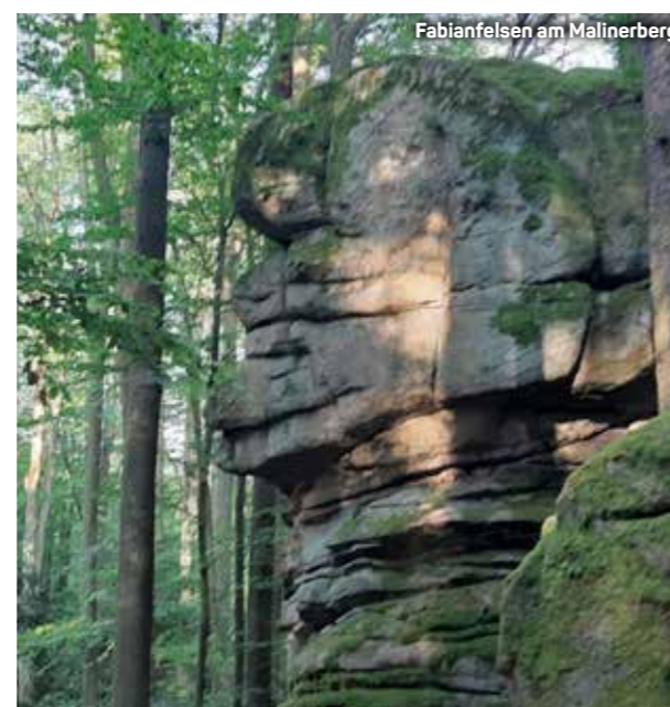
Fabianfelsen am Malinerberg
